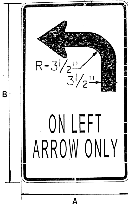
R17-3 NON-STANDARD (MODIFIED, STANDARD PLANS) ON LEFT ARROW ONLY
