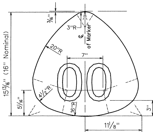
STATE ROUTE MARKER FOR GUIDE SIGNS
