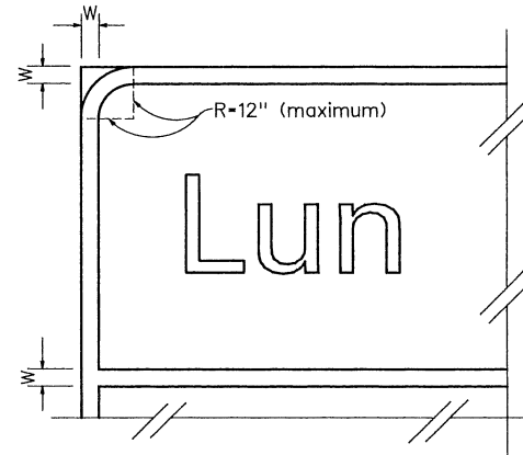
BORDER DETAIL FOR GUIDE SIGNS
