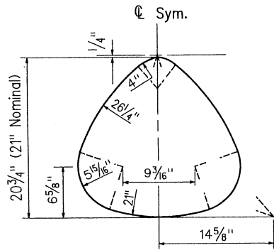
STATE ROUTE MARKER DETAIL
