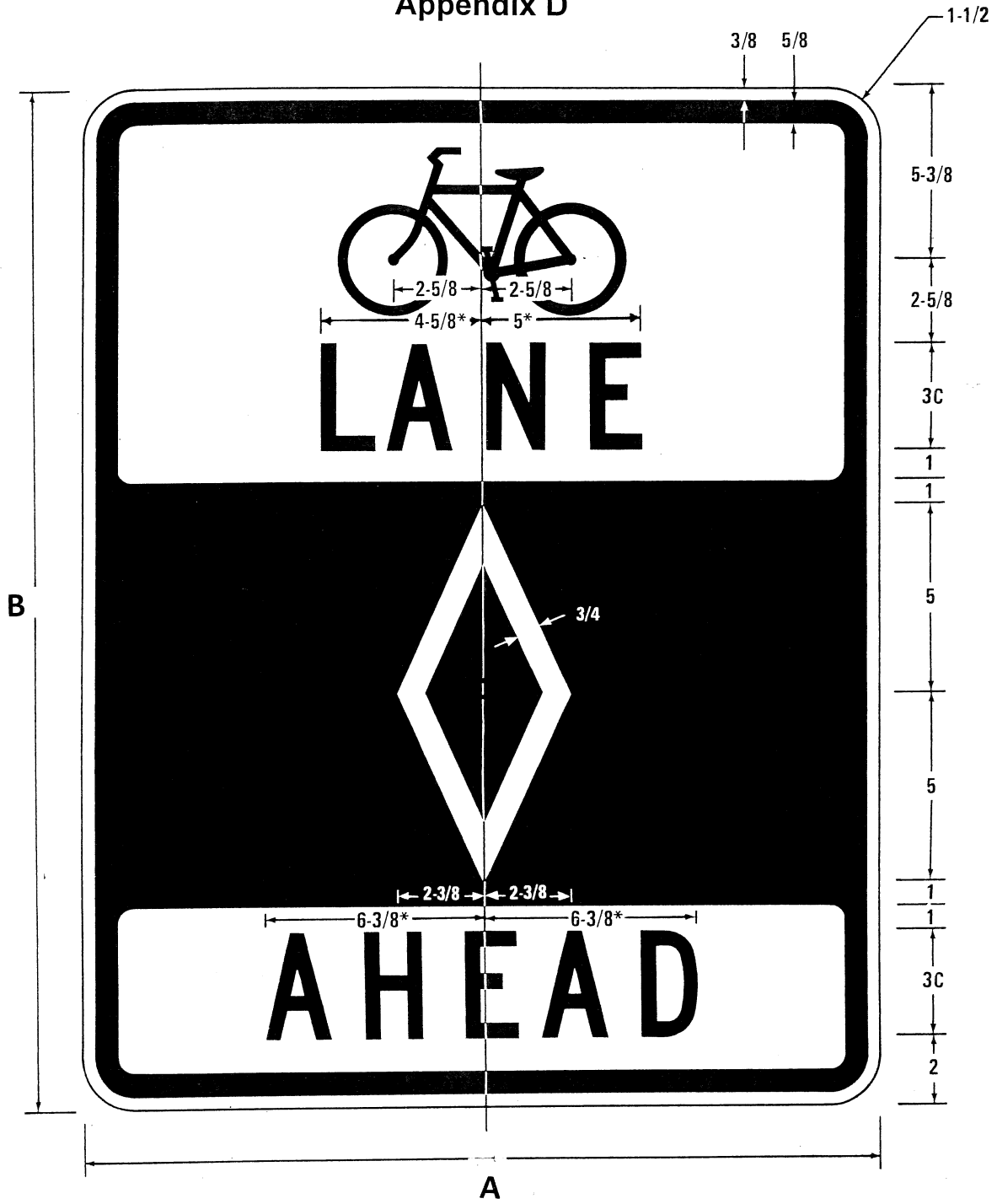
R3-16 NON-STANDARD BICYCLE (SYMBOL) LANE AHEAD
