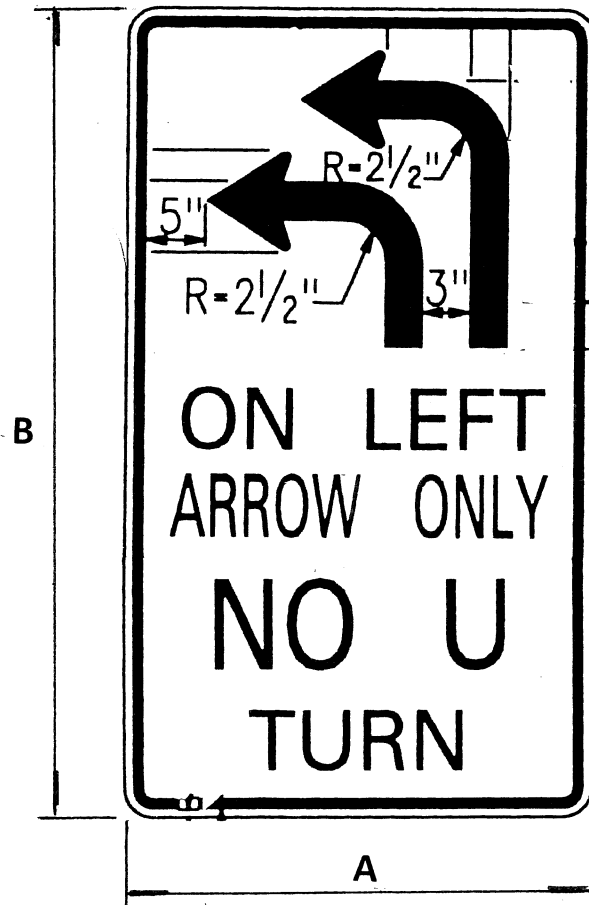
R17-4 NON-STANDARD (MODIFIED, STANDARD PLANS) ON LEFT ARROW ONLY NO U TURN
